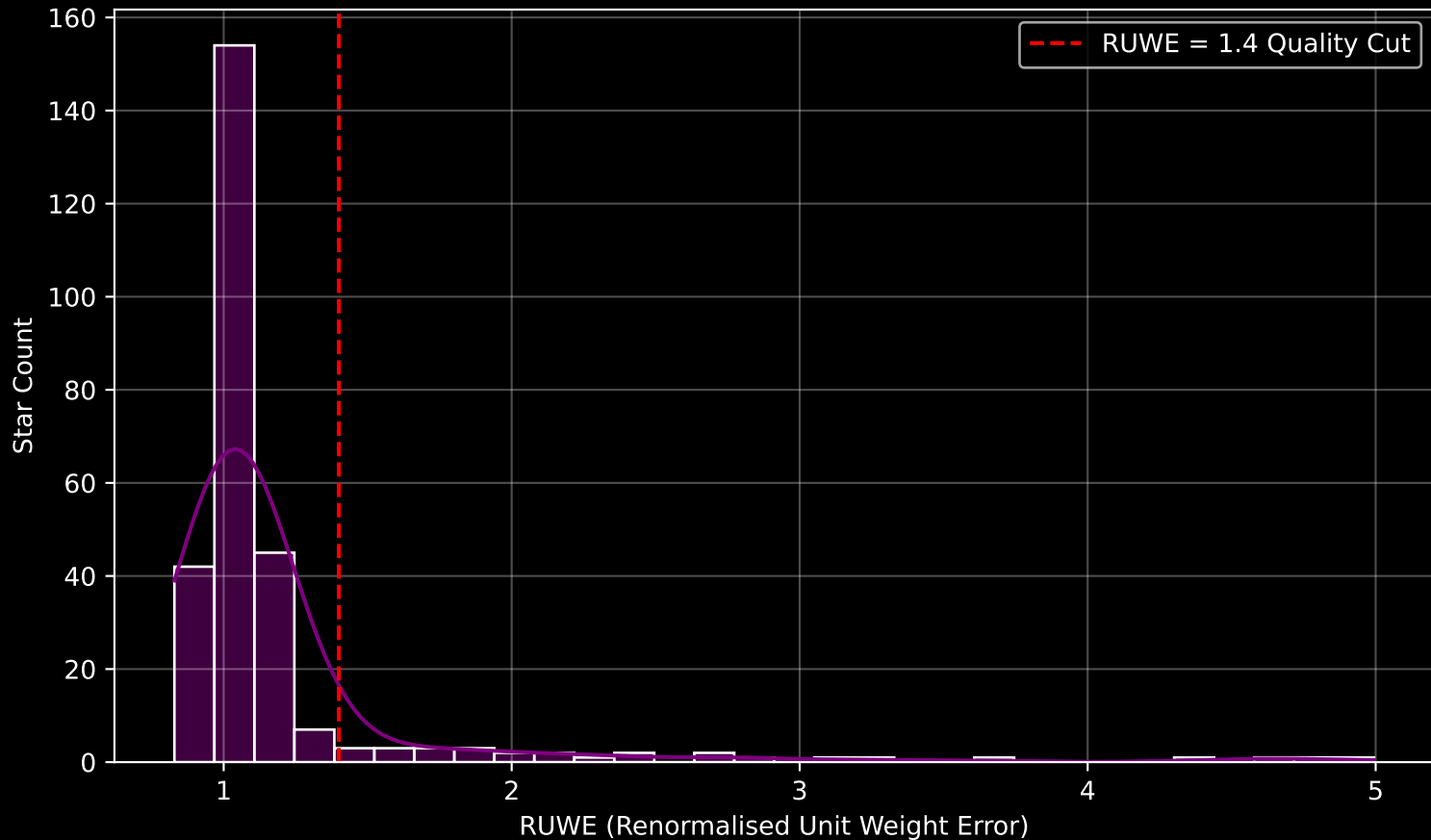
GALAH DR4 Field [9469] RUWE Distribution (n= 277)
