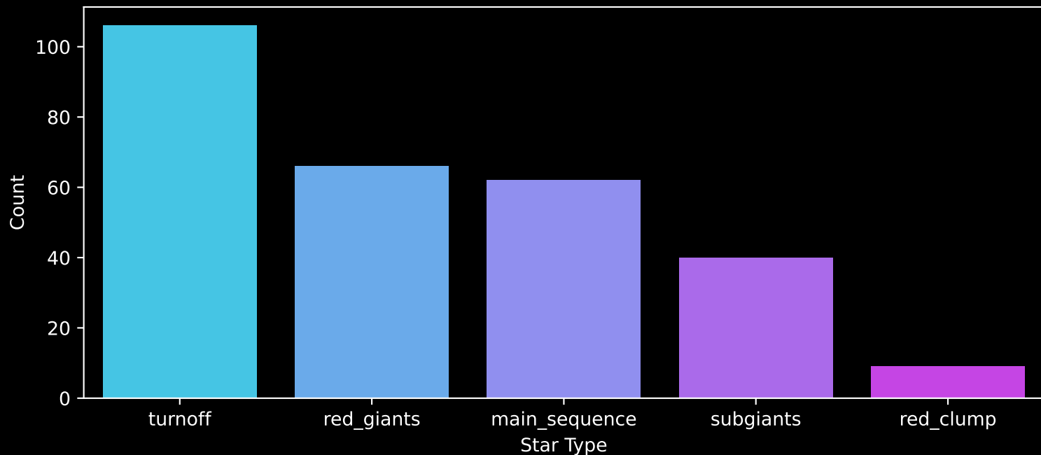
GALAH DR4 Field: [9469] Count plot of Star Type
